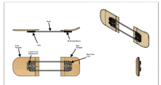
Luke Nelson – Compact Skateboard
